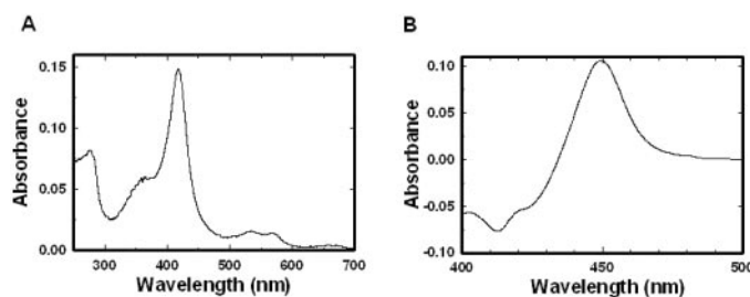
Fig. 1. Characterization of purified P450 2B6dH. A, absolute spectrum (250–700 nm). B, P450 reduced -CO difference spectrum (400–500 nm).
